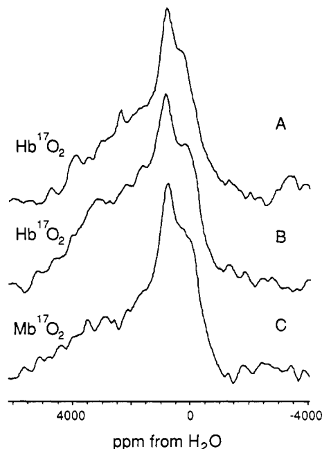
Figure 4. 8.45-T ^{17}\text{O} NMR spectra at 77 K of ^{17}\text{O}_2 hemoglobin and -myoglobin: (A) hemoglobin, frozen solution; (B) hemoglobin, polyethylene glycol microcrystals; (C) myoglobin, polyethylene glycol microcrystals.
